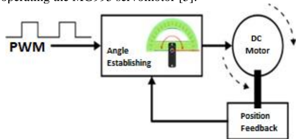
Fig 7. Block diagram of servo library.
