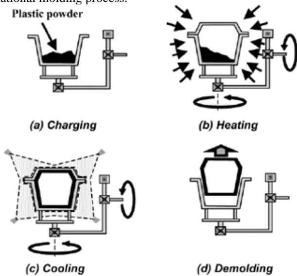
Fig 1. Rotational molding.
