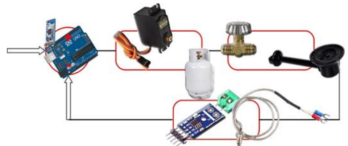
Fig 2. Prototype elements
