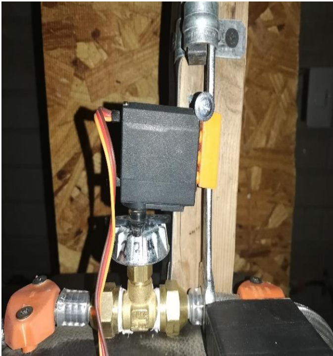
Fig 5. Valve prototype (actuator) for the gas control.
